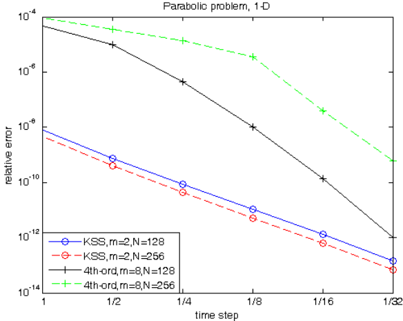
Figure 2: Estimates of relative error at t = 0.1 in solutions of (1) computed using a 4th-order method based on an exponential integrator [10] with 8 Lanczos iterations, and a 2-node block KSS method. Both methods compute solutions on an N -point grid, with time step \Delta t , for various values of N and \Delta t .
