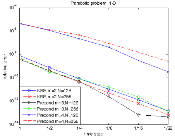
Figure 1: Estimates of relative error at t = 0.1 in solutions of (1) computed using preconditioned exponential integrator [19] with 4 and 8 Lanczos iterations, and a 2-node block KSS method. All methods compute solutions on an N -point grid, with time step \Delta t , for various values of N and \Delta t .
