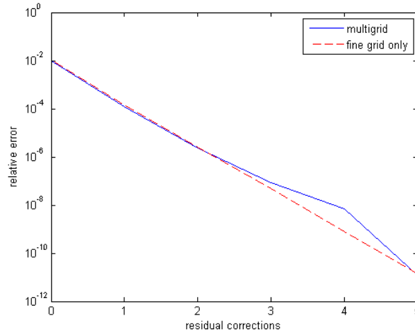
FIGURE 4. Relative error in solutions to Poisson’s equation (24), (25), (26) computed by 2-node block KSS methods with residual correction, on multiple grids with N = 32, 64, 128, 256, 512, 1024 grid point (blue solid curve) and a single grid with N = 1024 grid points (red dashed curve).
