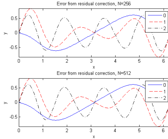
FIGURE 3. Error in computed solutions to a 1-D analogue of (19) after zero (solid blue curve), one (dashed red curve), and two (dotted-dashed black curve) iterations of residual correction in conjunction with a 2-node block KSS method on a 256-point grid (top plot) and a 512-point grid (bottom plot).
